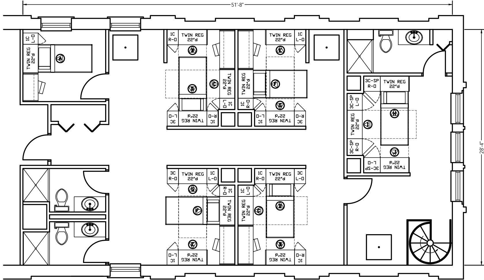
PLAN VIEW
