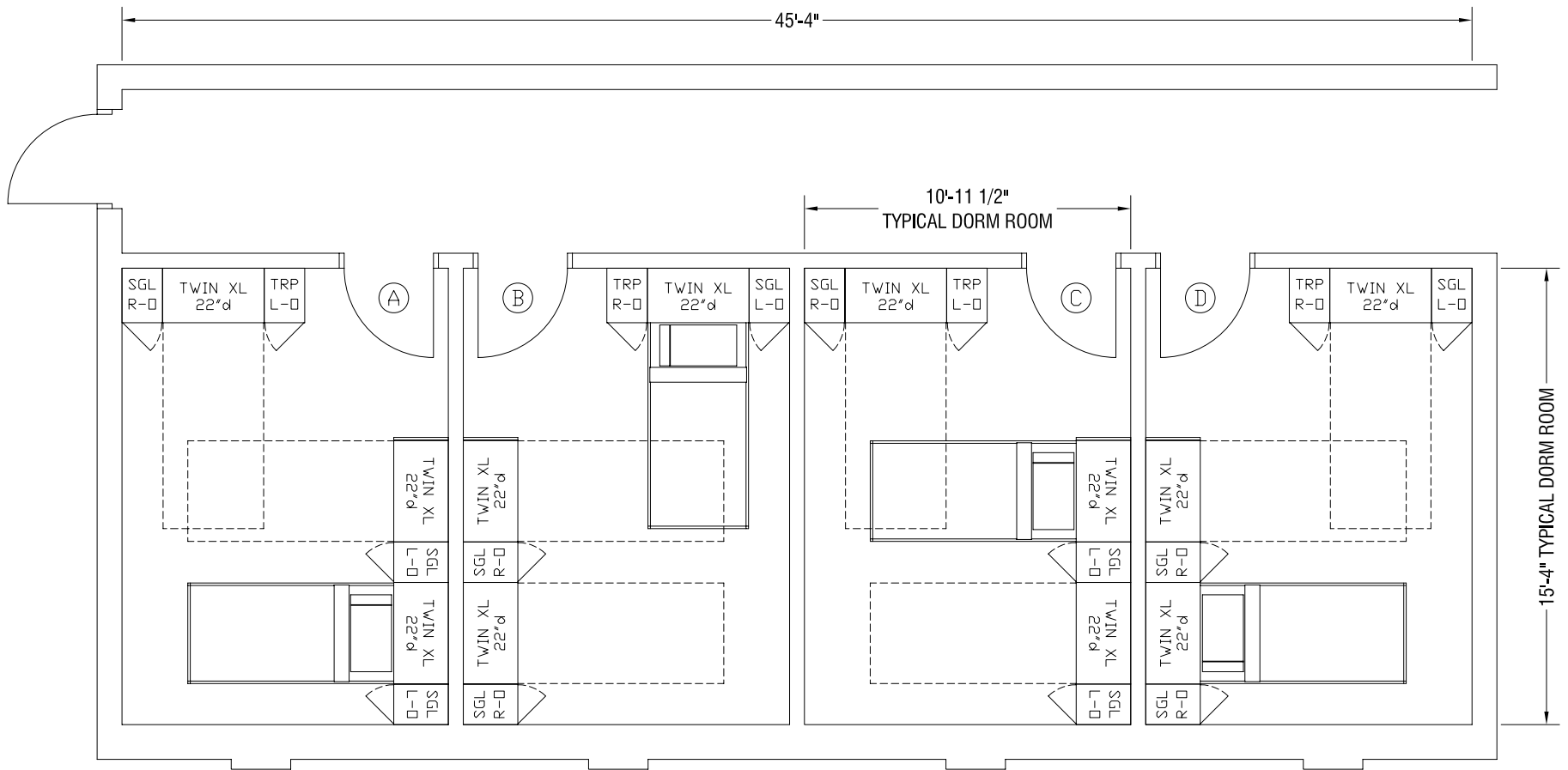
PLAN VIEW, DORM ROOM CUBICLES
